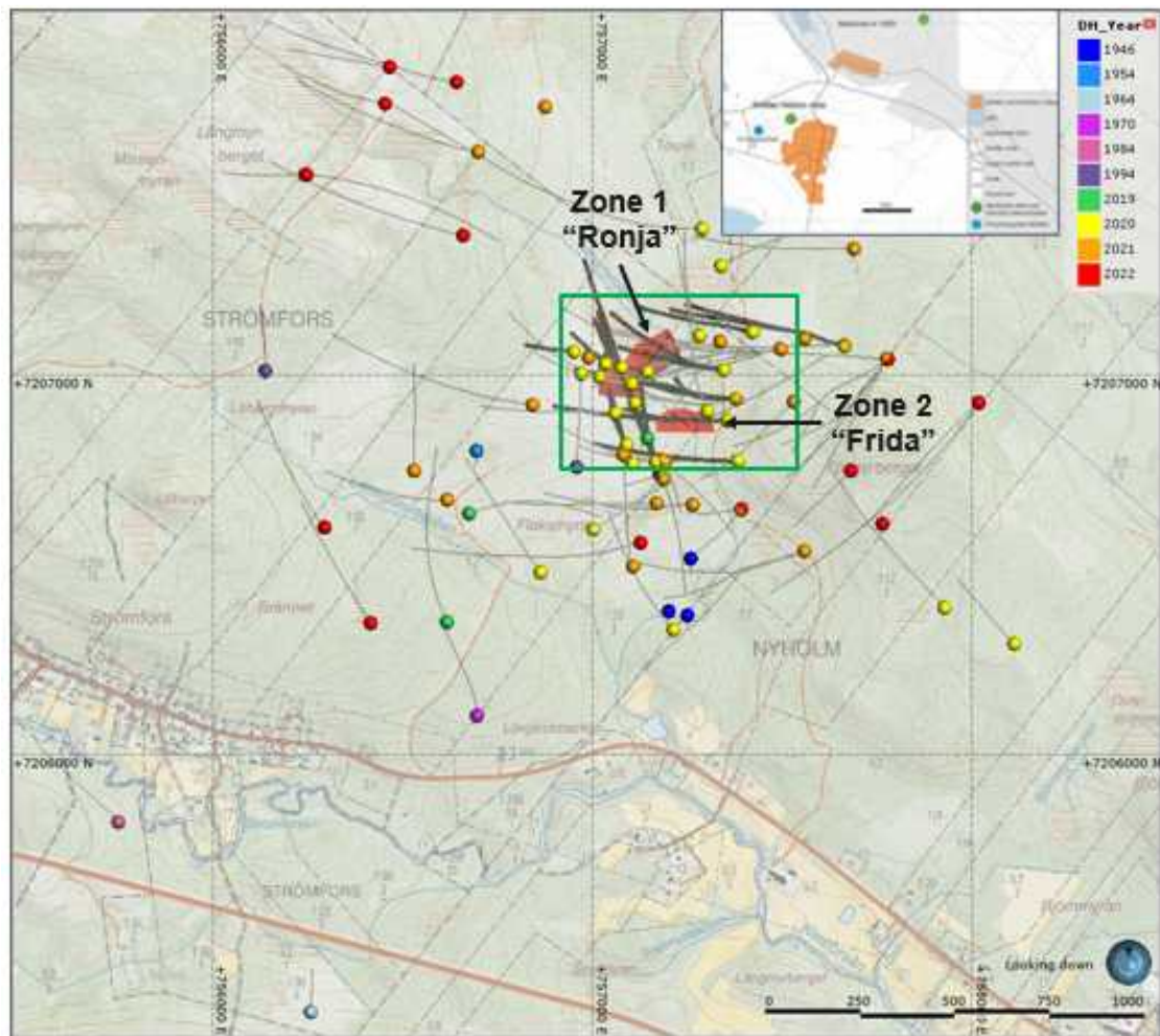
Figure 3.2 Exploration drilling over the Strömfors area. Drillhole collars are coloured by year completed. The green box indicates the mineral resource area for December 31, 2022 (where drillholes used in this estimation are highlighted in dark grey).
